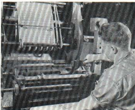
Printer replenishes ink fountain of a steel plate printing press and checks even spread of ink on roller. Stamps above have passed through press and are on conveyor belt to sheet-cutting operation.
