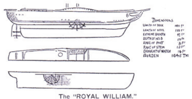
Drawings of the Royal William
