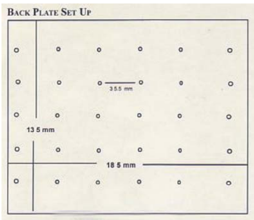
Plate with dowels to receive the small plates.
